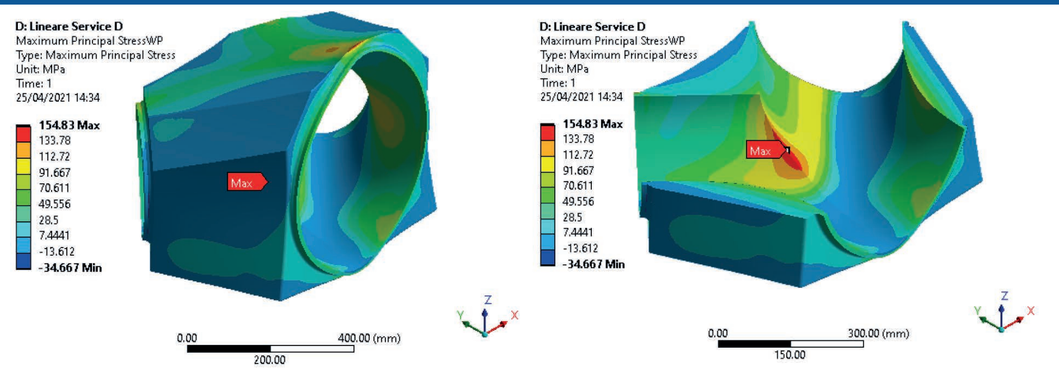
PRINCIPAL STRESS
